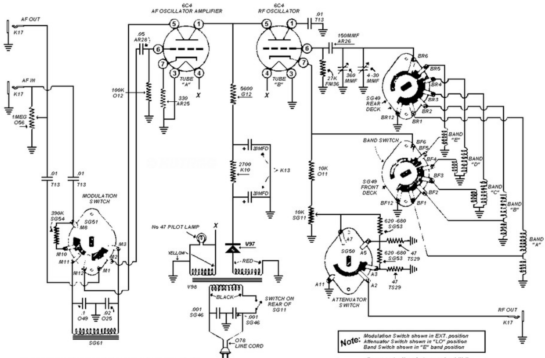
HEATHKIT SIGNAL GENERATOR MODEL SG-6
