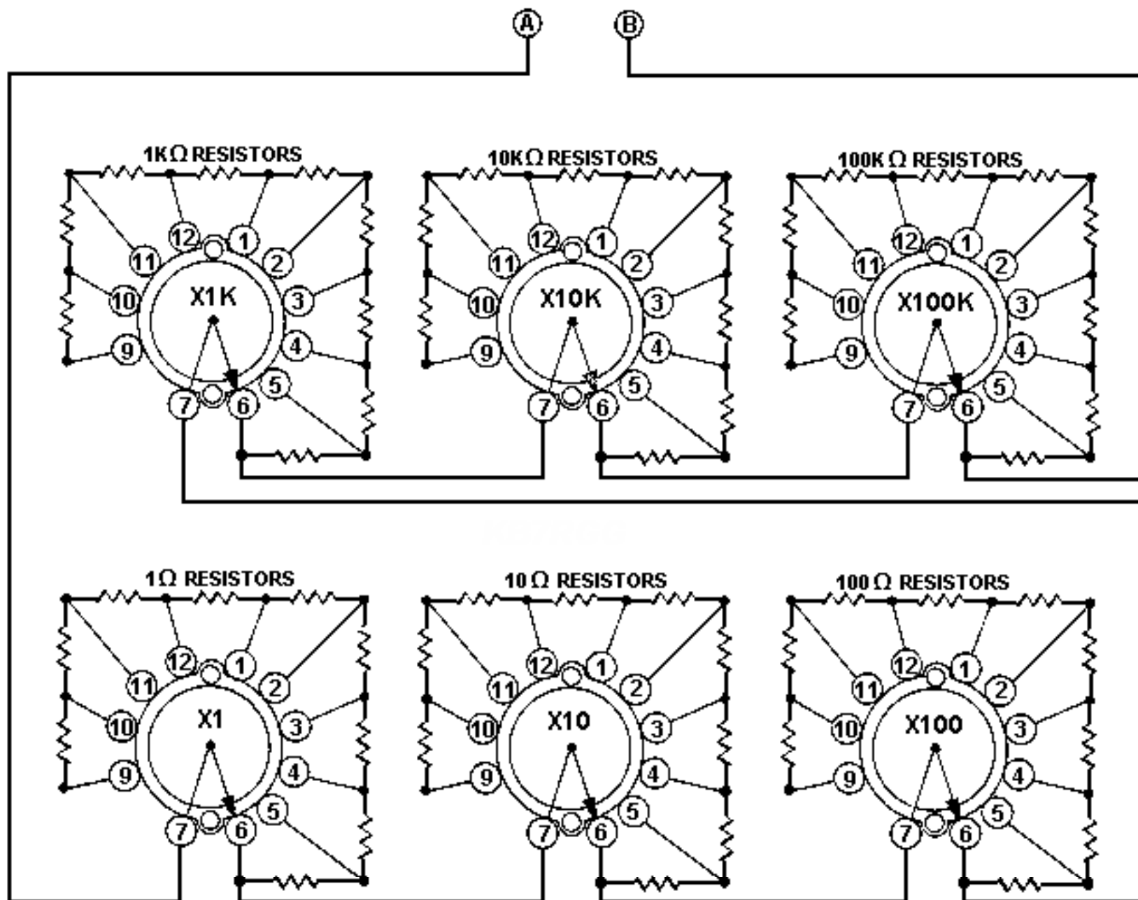
SCHEMATIC DIAGRAM MODEL IN-11
