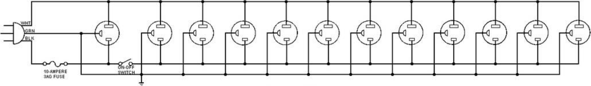
SCHEMATIC OF THE HEATHKIT OUTLET BOX MODEL HD-1274
