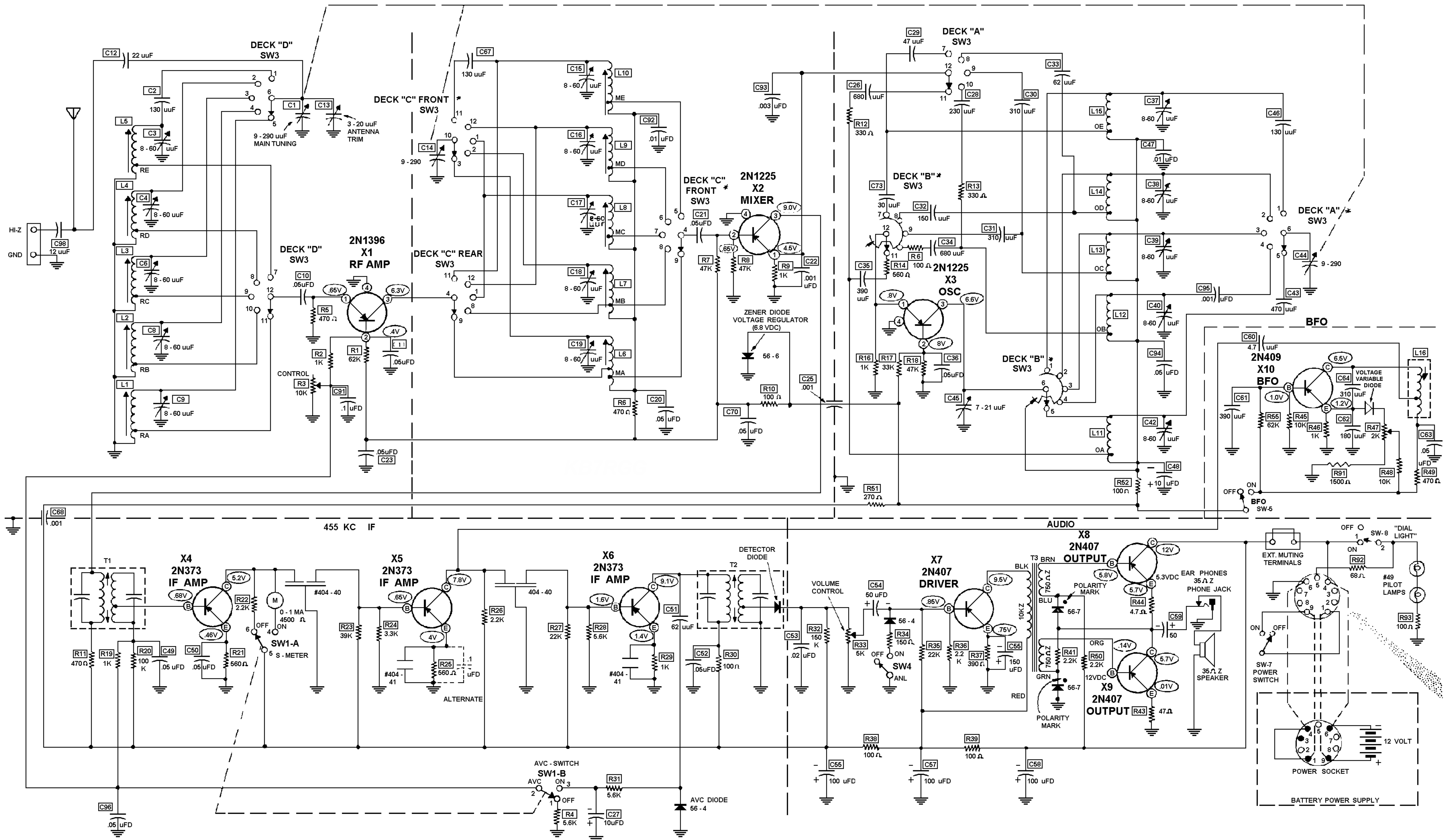
HEATHKIT GC-1A
