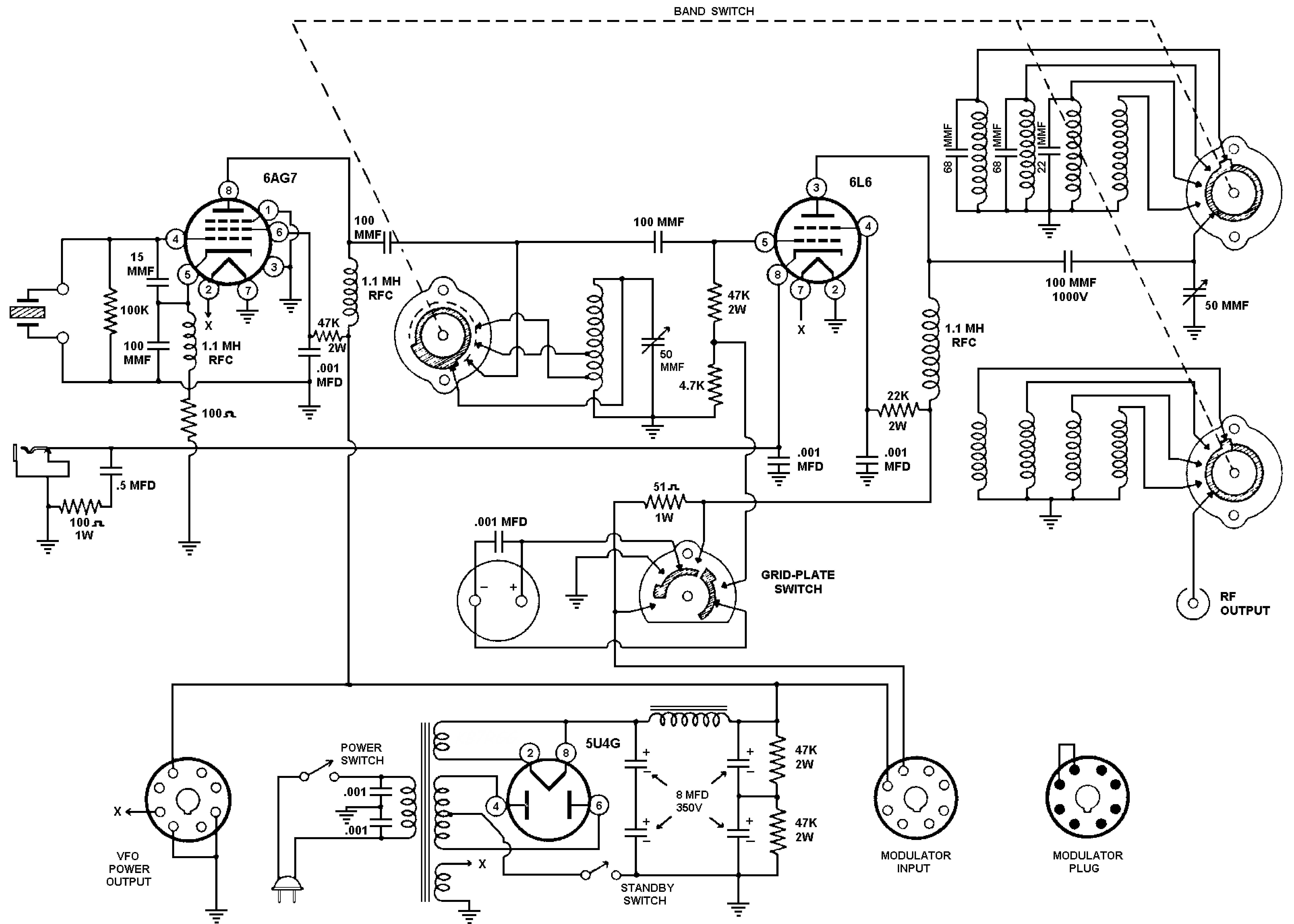
HEATHKIT AMATEUR TRANSMITTER MODEL AT-1
