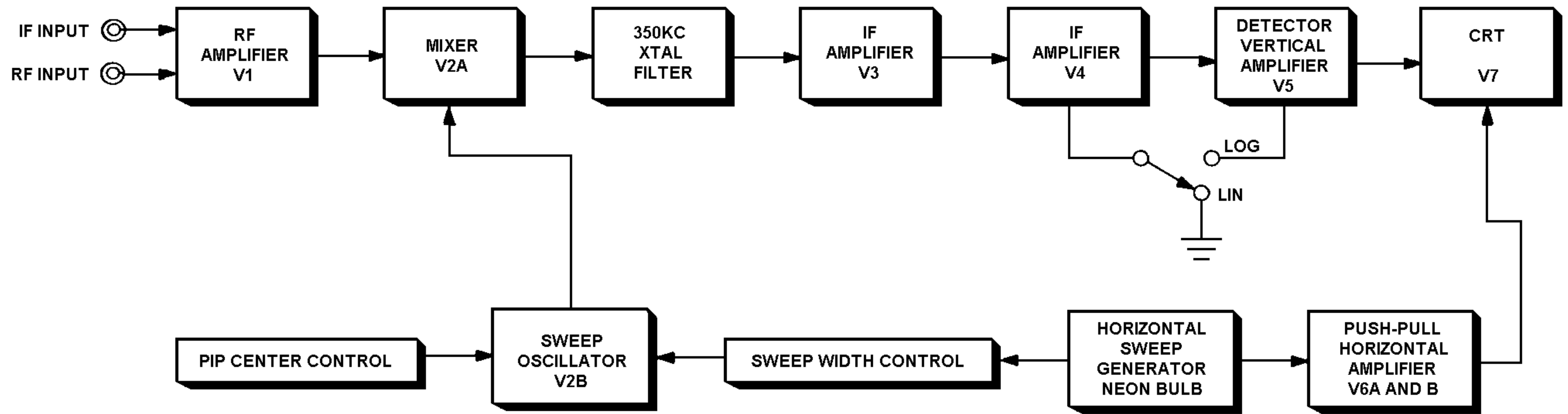
HEATHKIT SB-620 BLOCK DIAGRAM
