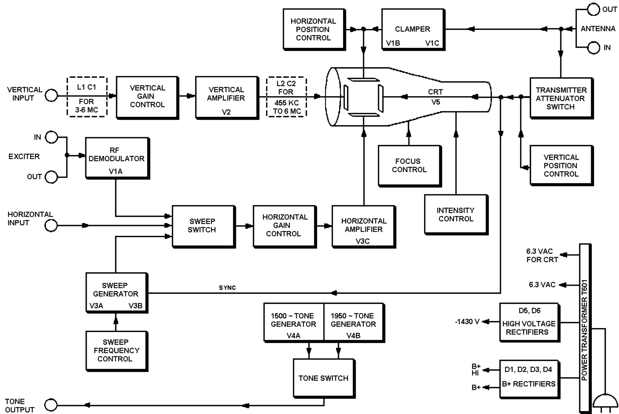
HEATHKIT SB-610 BLOCK DIAGRAM
