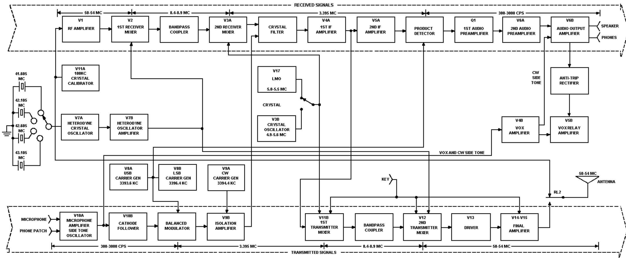
HEATHKIT SB-110 BLOCK DIAGRAM
