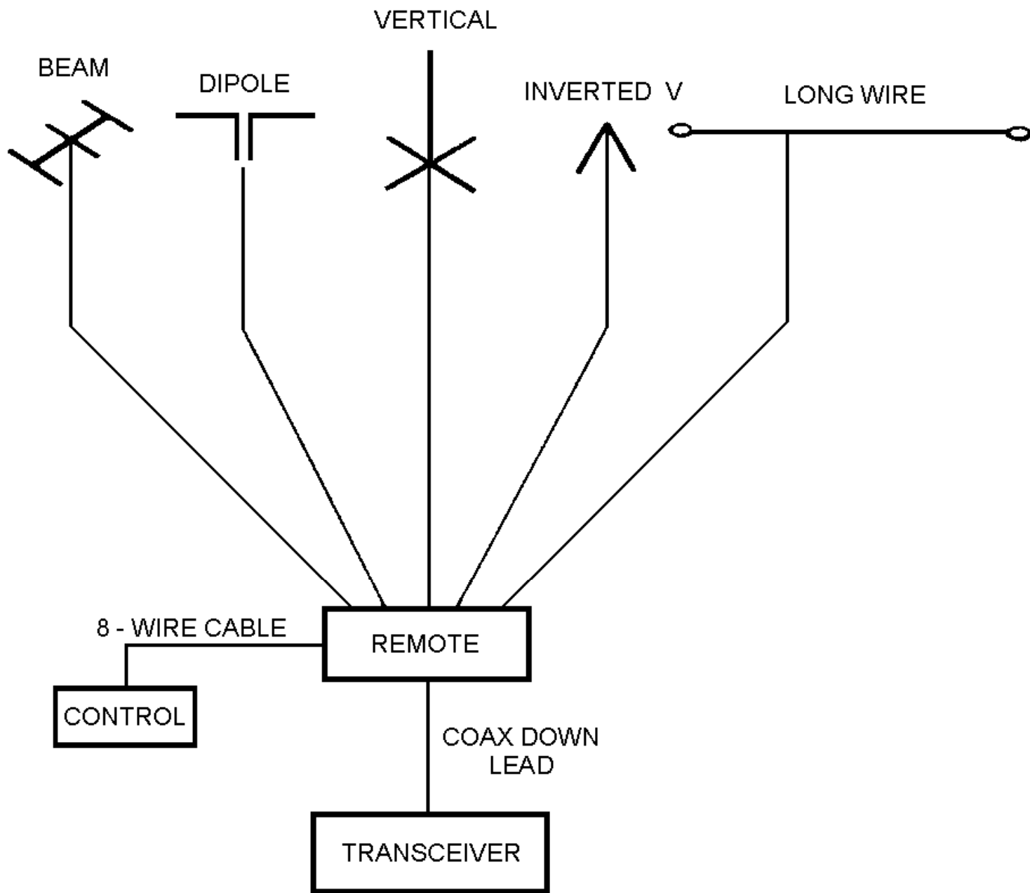
Heathkit SA-1480 Block Diagram
