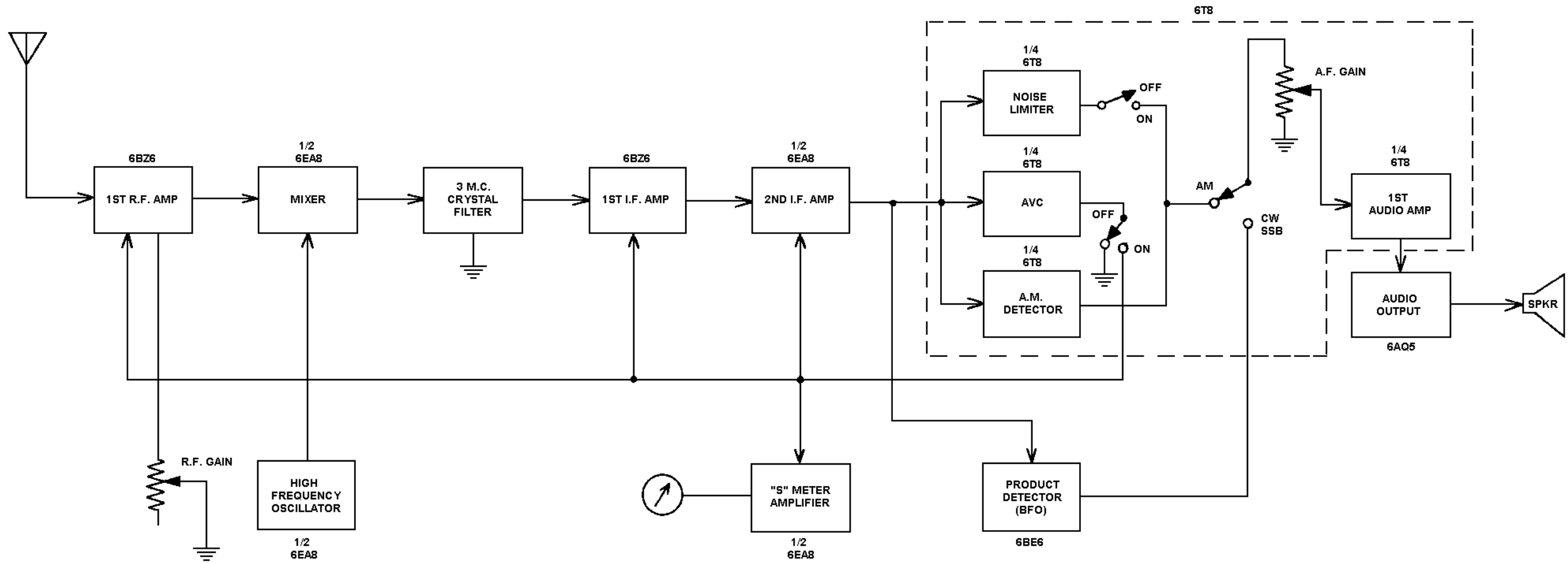
HEATHKIT MR-1 BLOCK DIAGRAM
