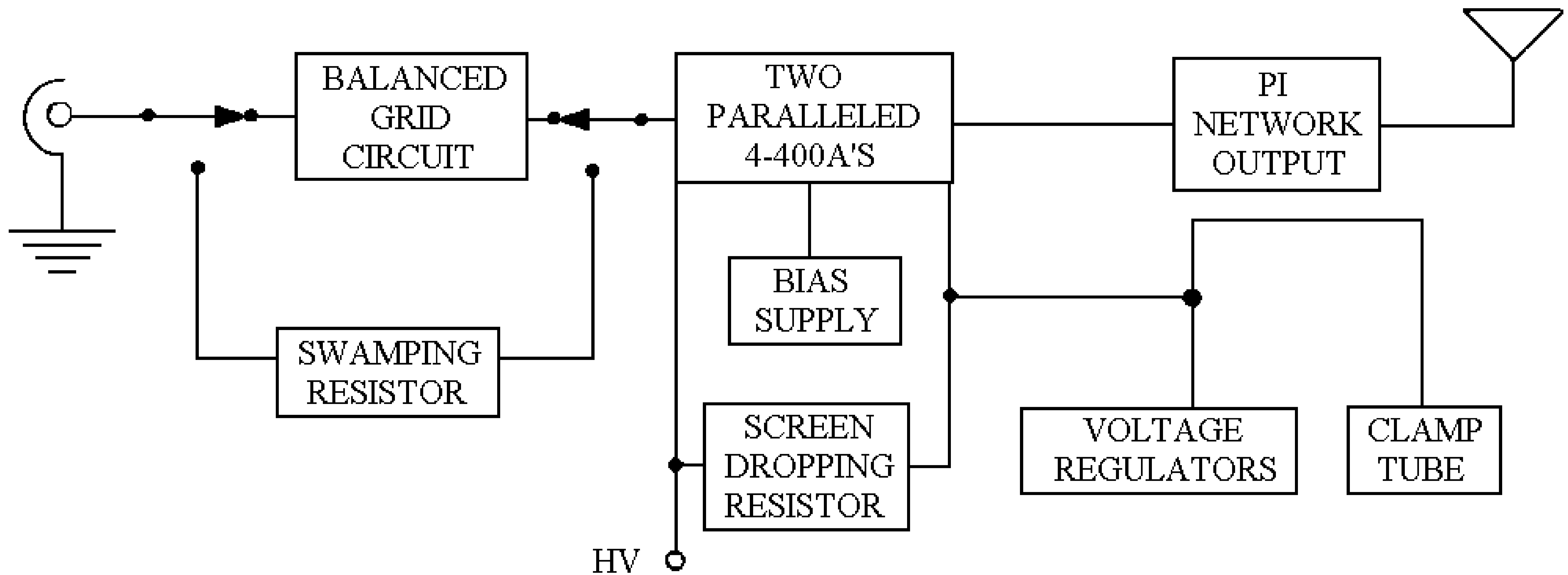
HEATHKIT KL-1 BLOCK DIAGRAM
