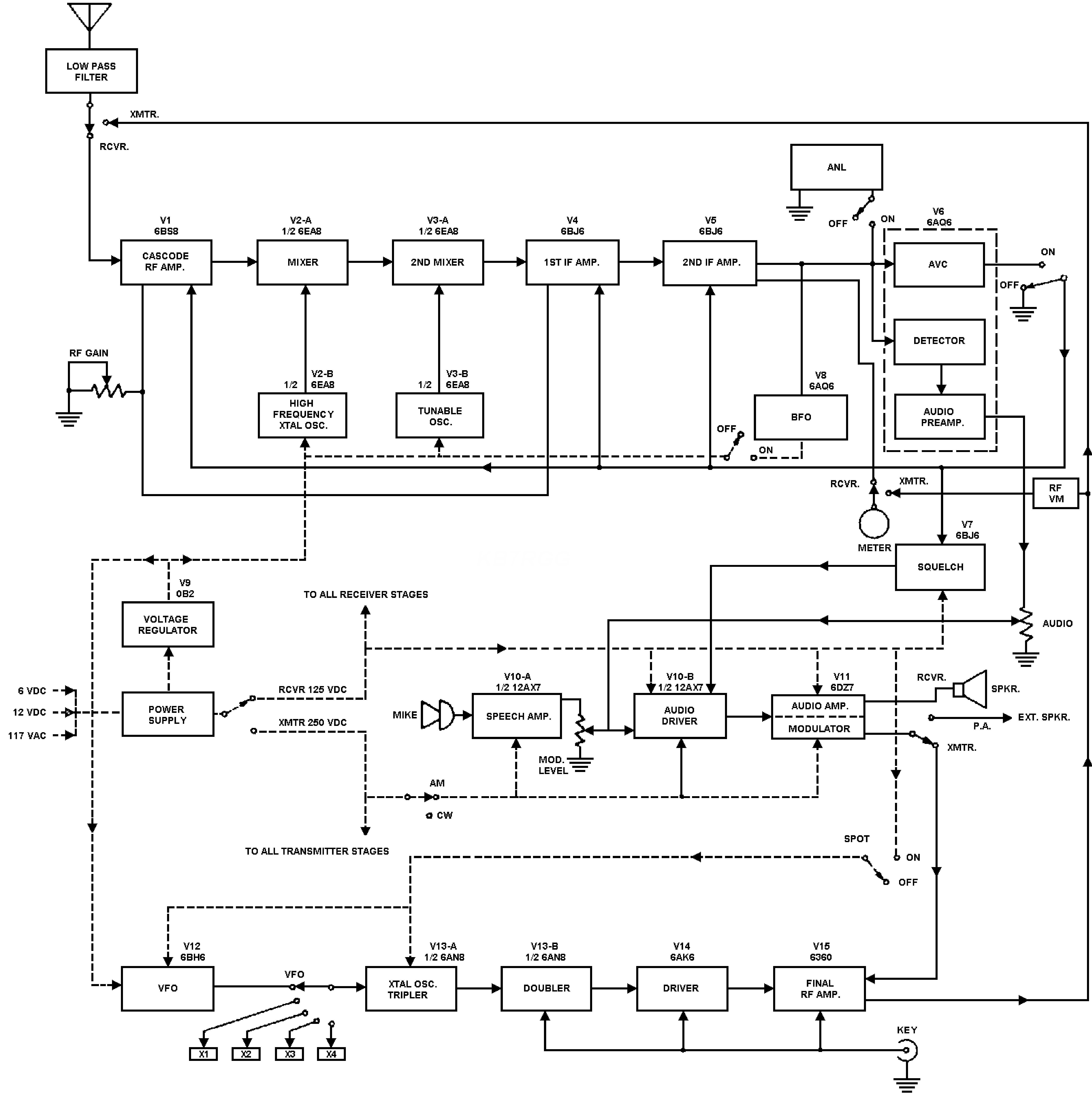
HEATHKIT HW-10 BLOCK DIAGRAM
