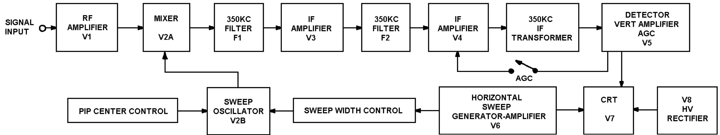
HEATHKIT HO-13 BLOCK DIAGRAM
