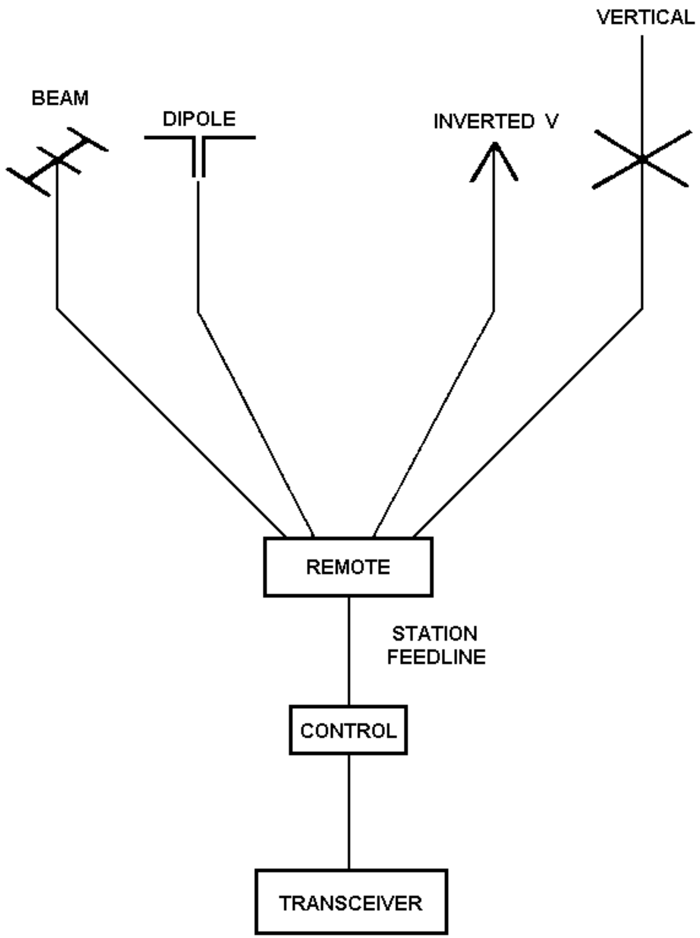
HEATHKIT HD-1481 BLOCK DIAGRAM
