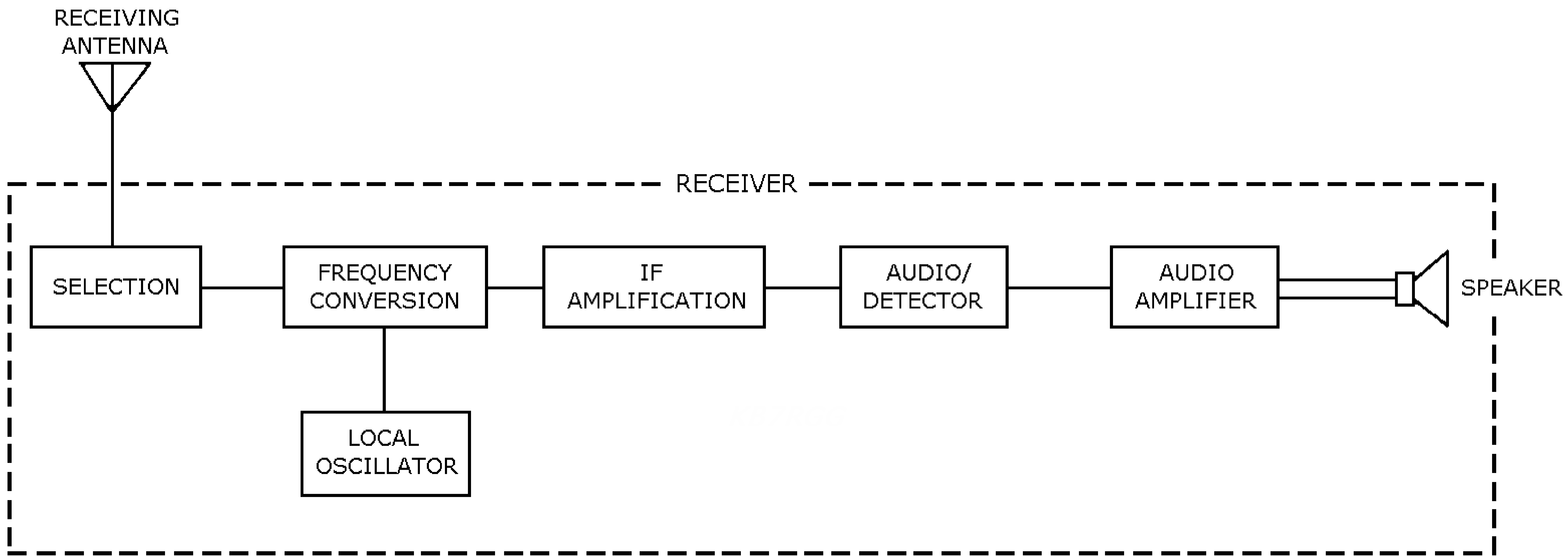
HEATHKIT GR-64 BLOCK DIAGRAM
