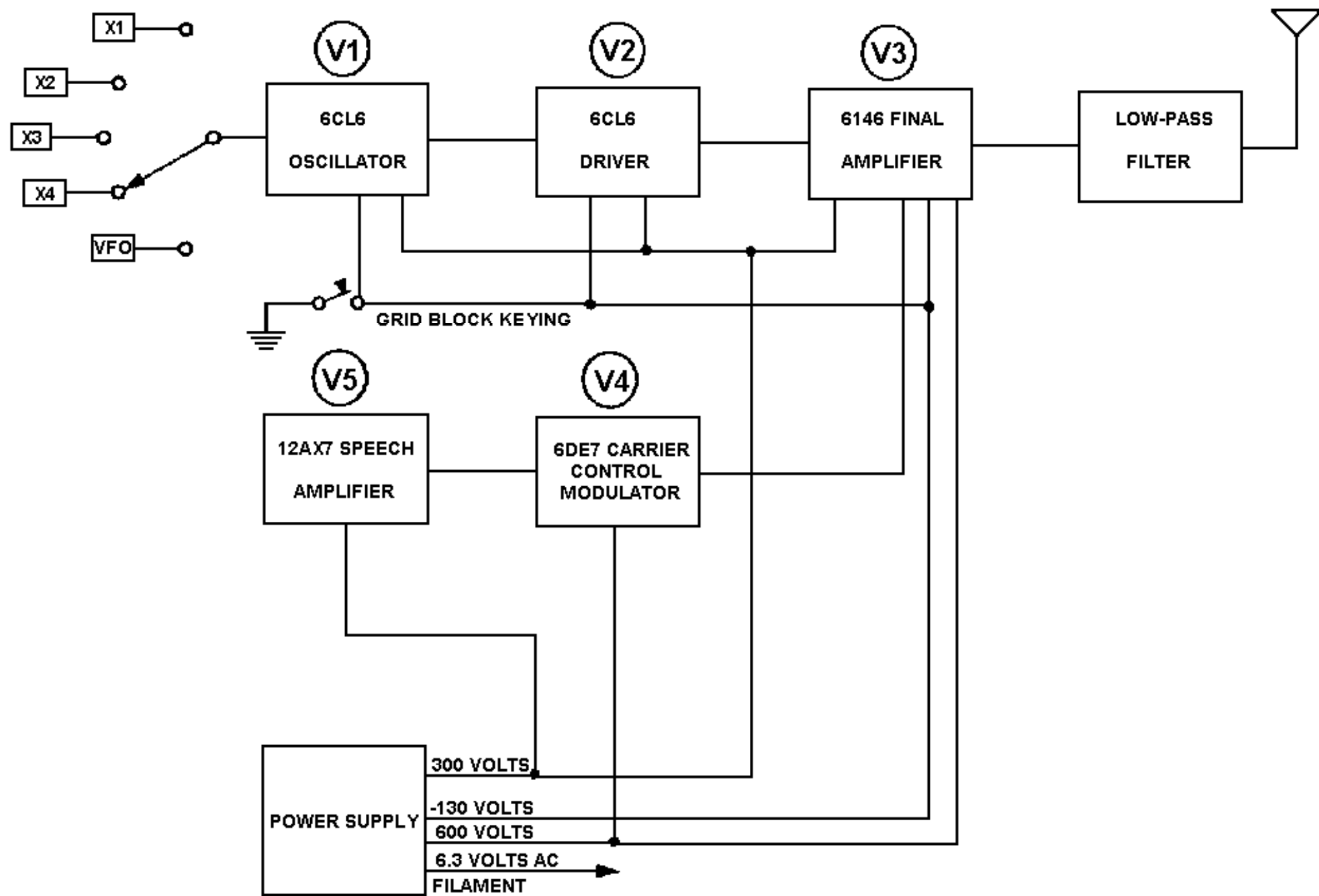
HEATHKIT DX-60 BLOCK DIAGRAM
