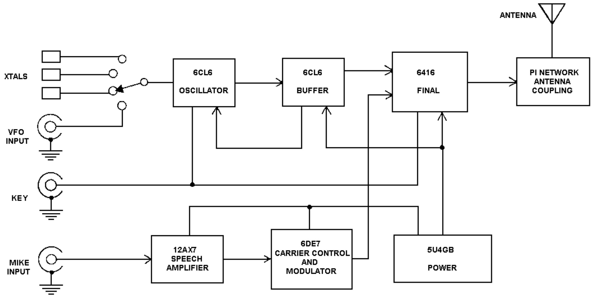
HEATHKIT DX-40 BLOCK DIAGRAM
