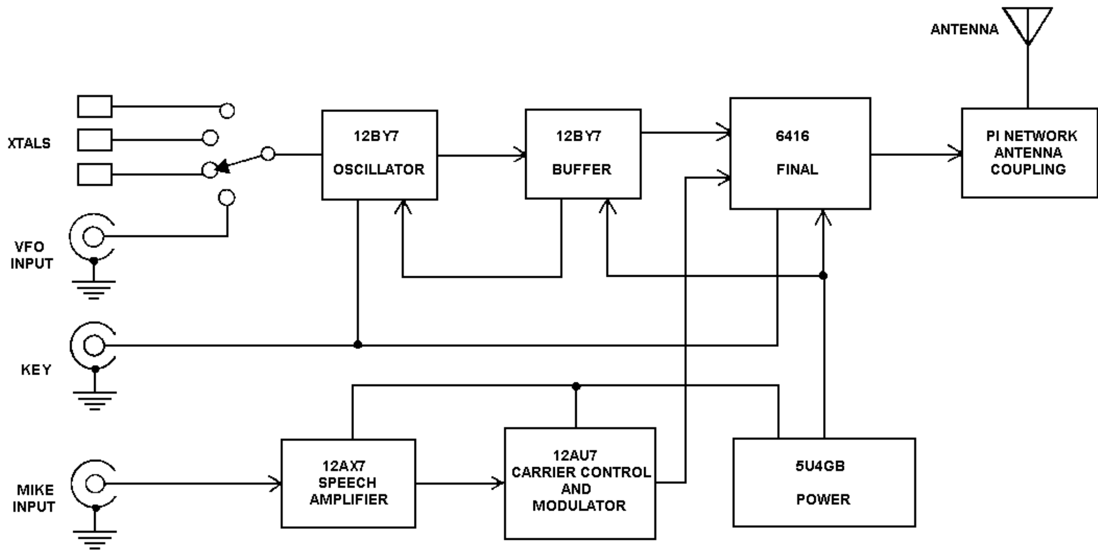
HEATHKIT DX-35 BLOCK DIAGRAM
