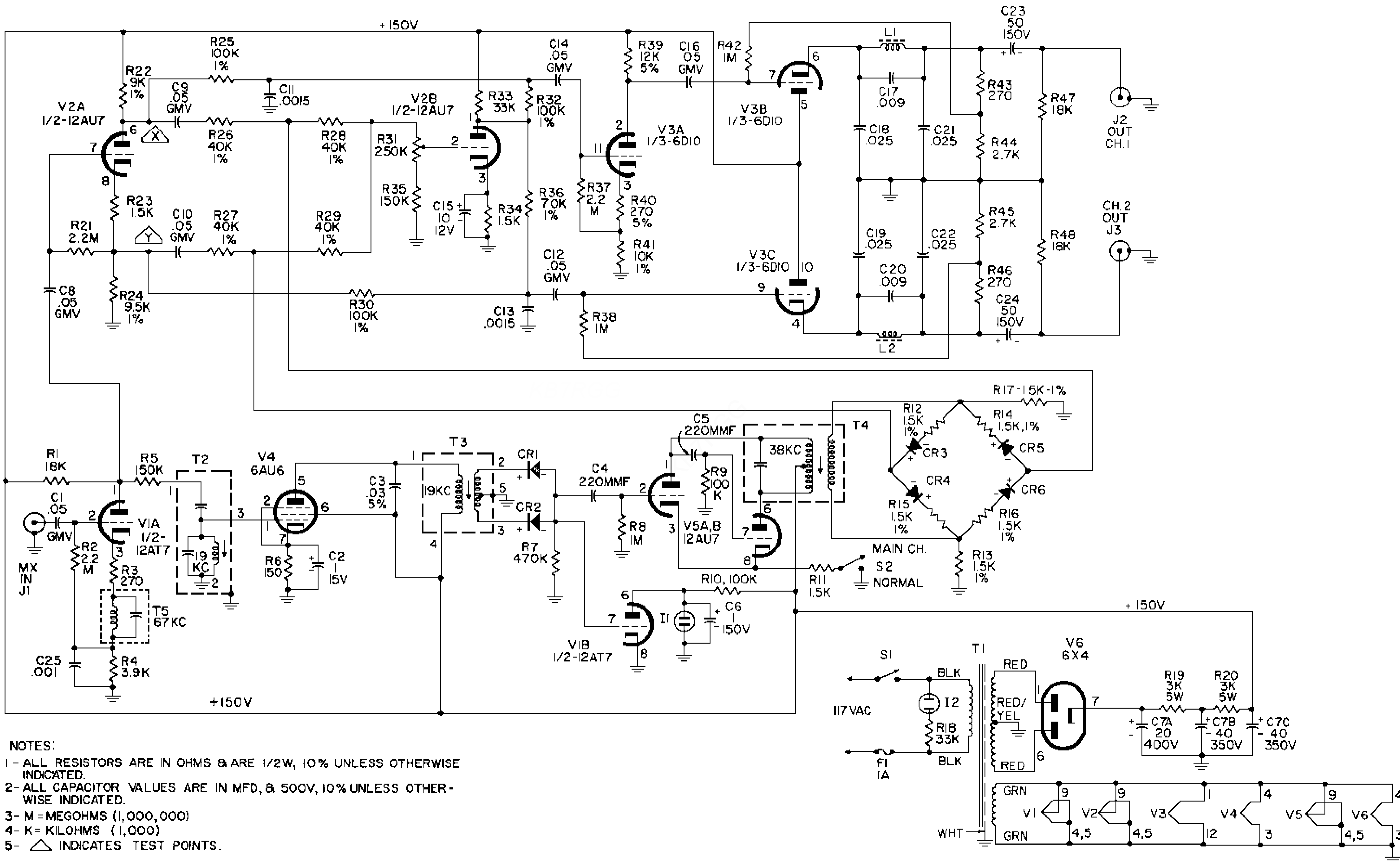
MX-99 Schematic Diagram
