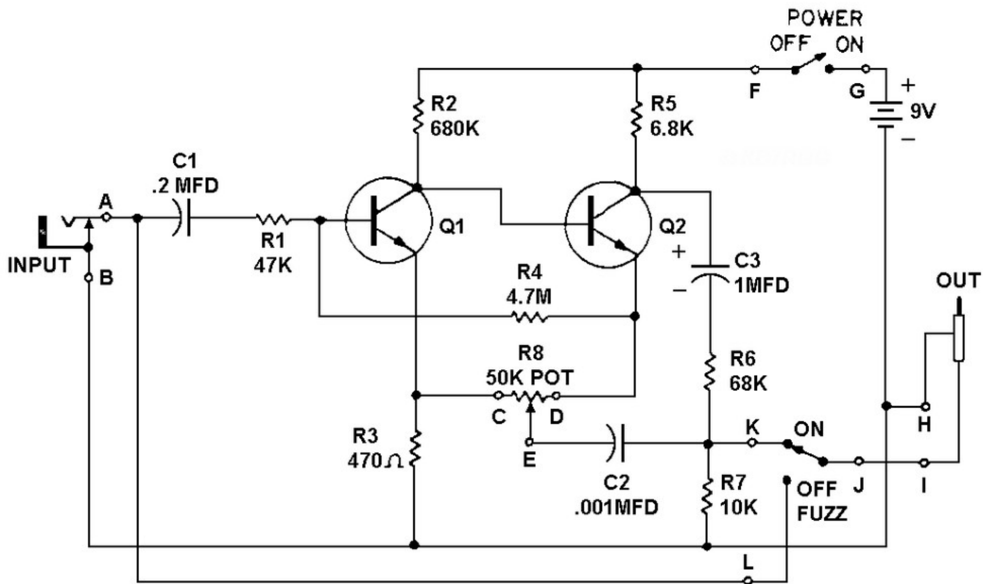
EICO EC2500 GUITAR FUZZ BOX
