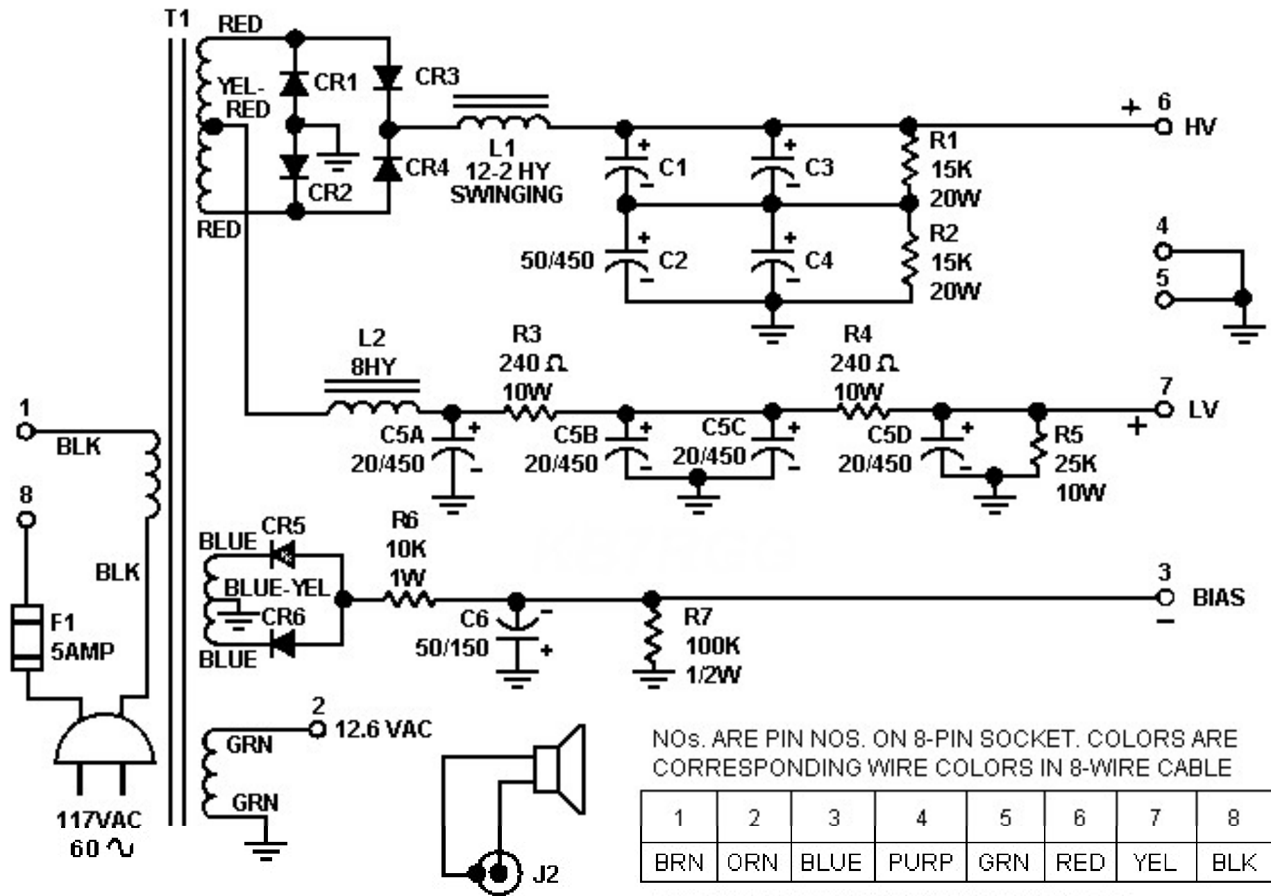
EICO 751 SCHEMATIC DIAGRAM
