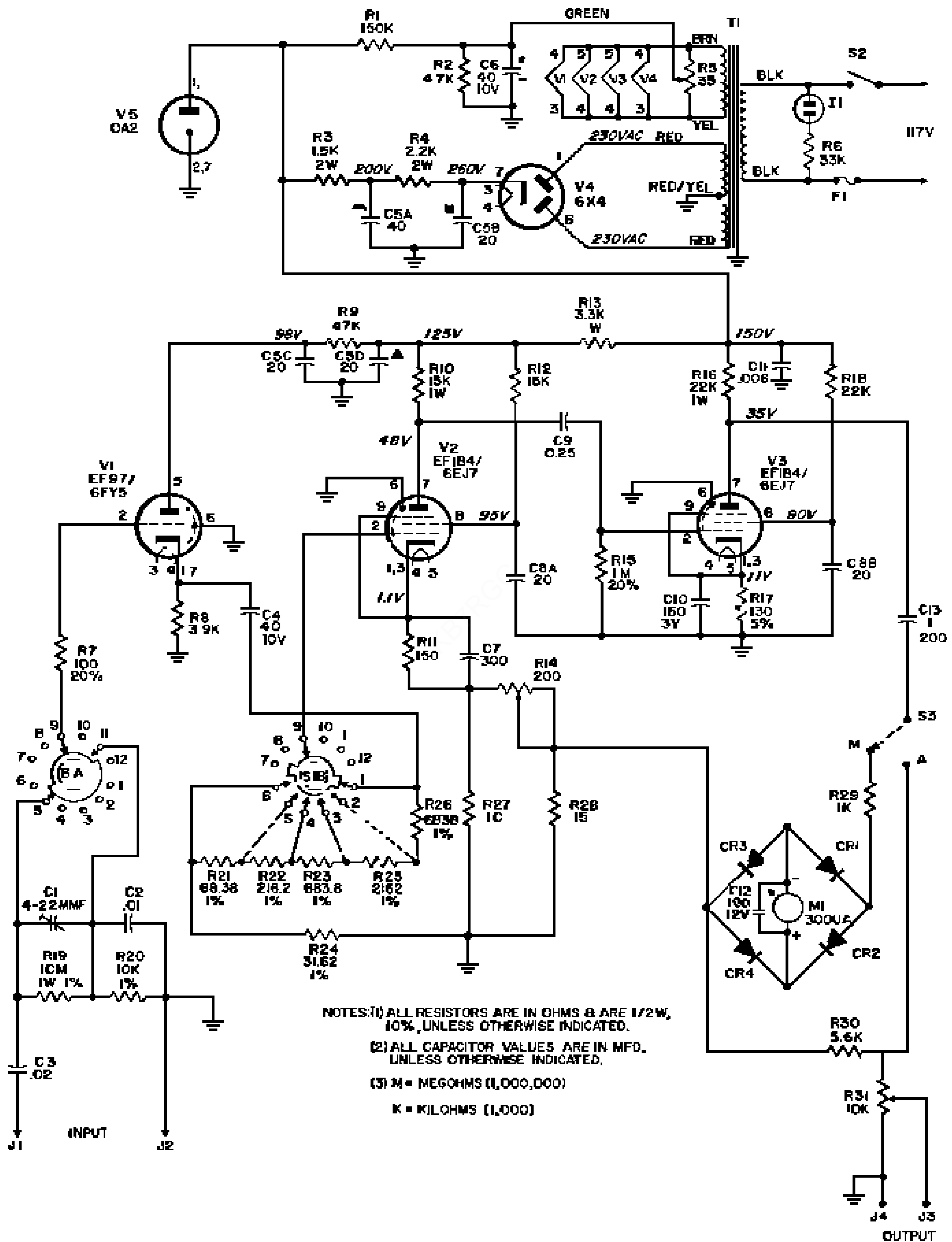
Figure 4-2. 250 Schematic Diagram
