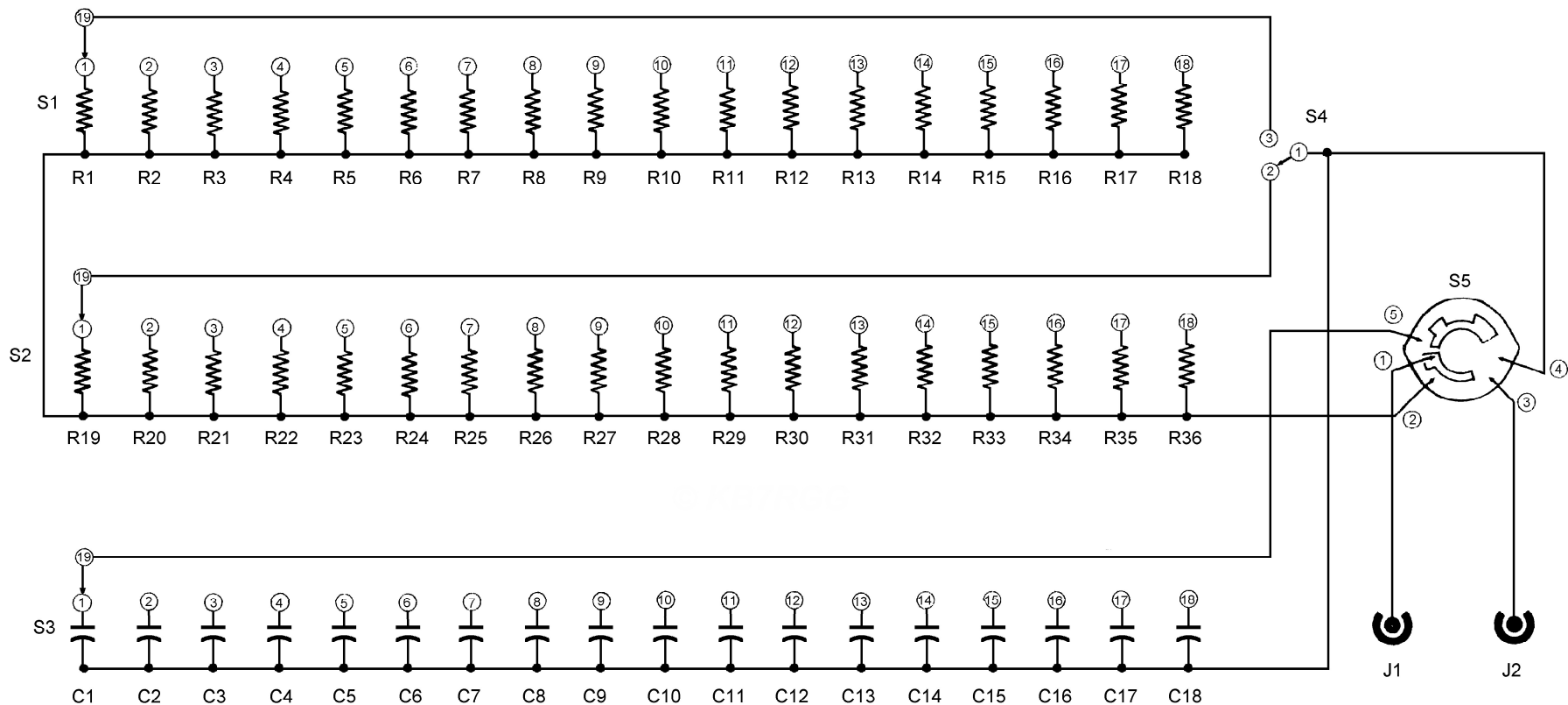
MODEL 1140 SERIES-PARALLEL R-C COMBINATION BOX SCHEMATIC DIAGRAM
