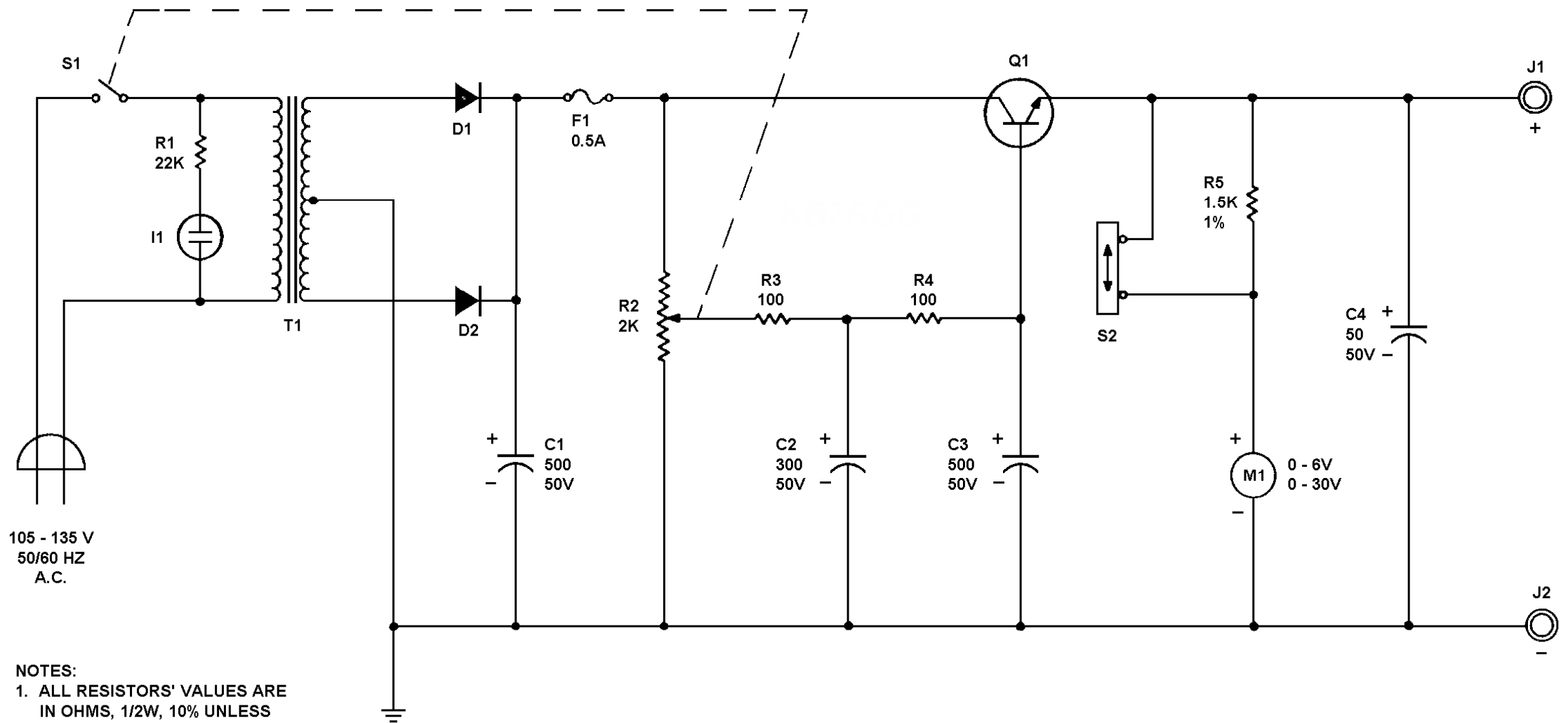
Eico Model 1020 Power Supply Schematic
