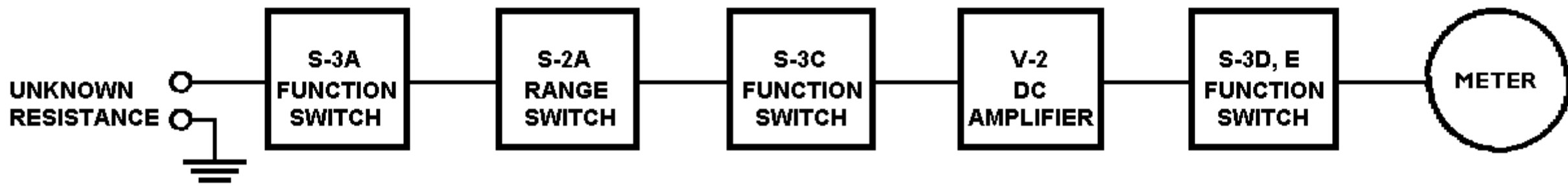
EICO 221 BLOCK DIAGRAM
