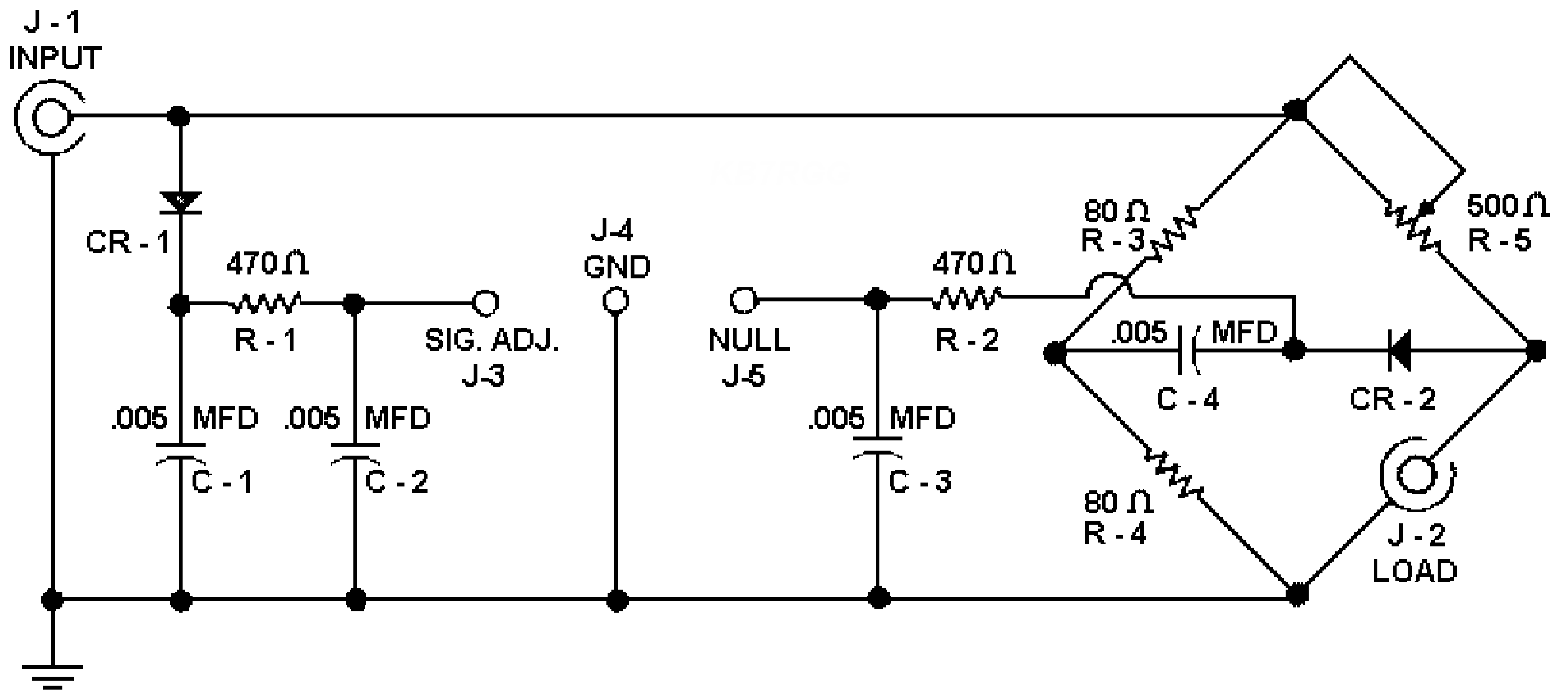
KNIGHT Z52 SWR and Z-Bridge
