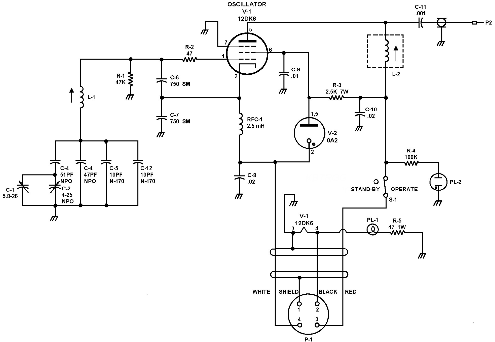
KNIGHT V107 SCHEMATIC DIAGRAM
