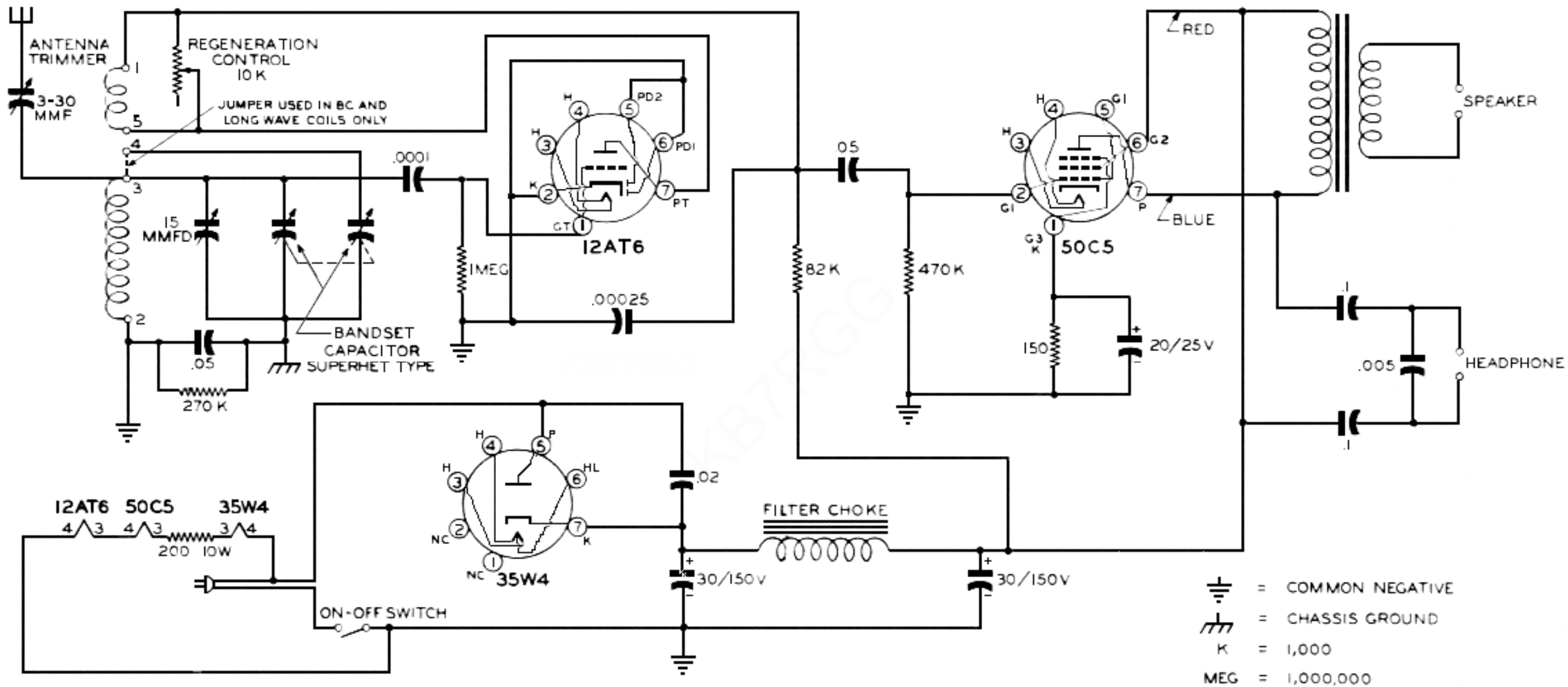
SCHEMATIC DIAGRAM OCEAN HOPPER 740
