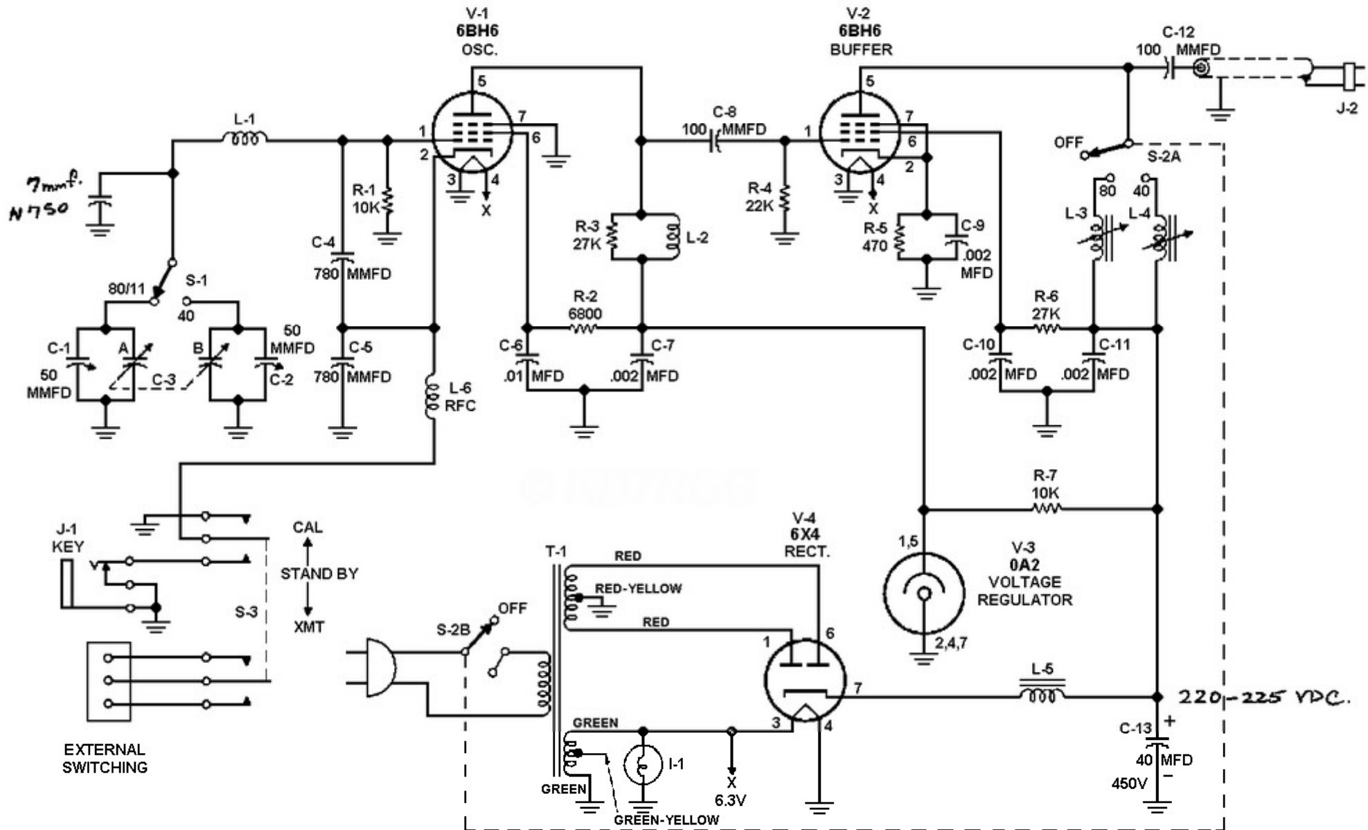
SCHEMATIC DIAGRAM - KNIGHT VFO
