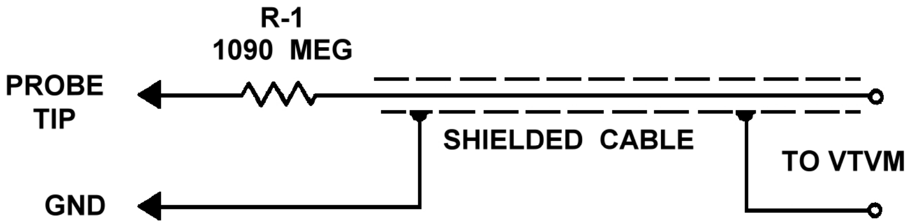
Knight 83Y126 High Voltage Probe
