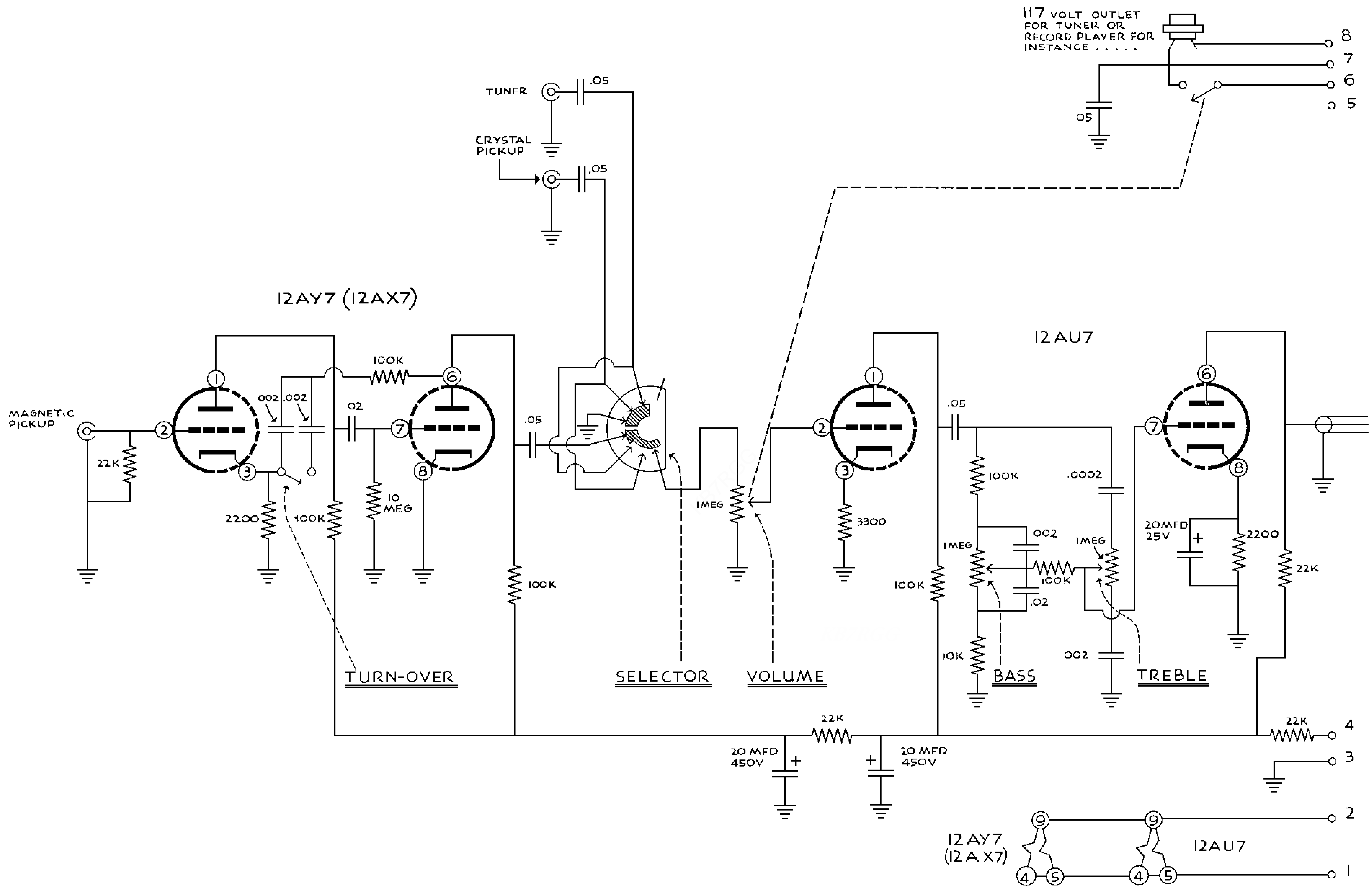
PREAMPLIFIER CIRCUIT DIAGRAM
