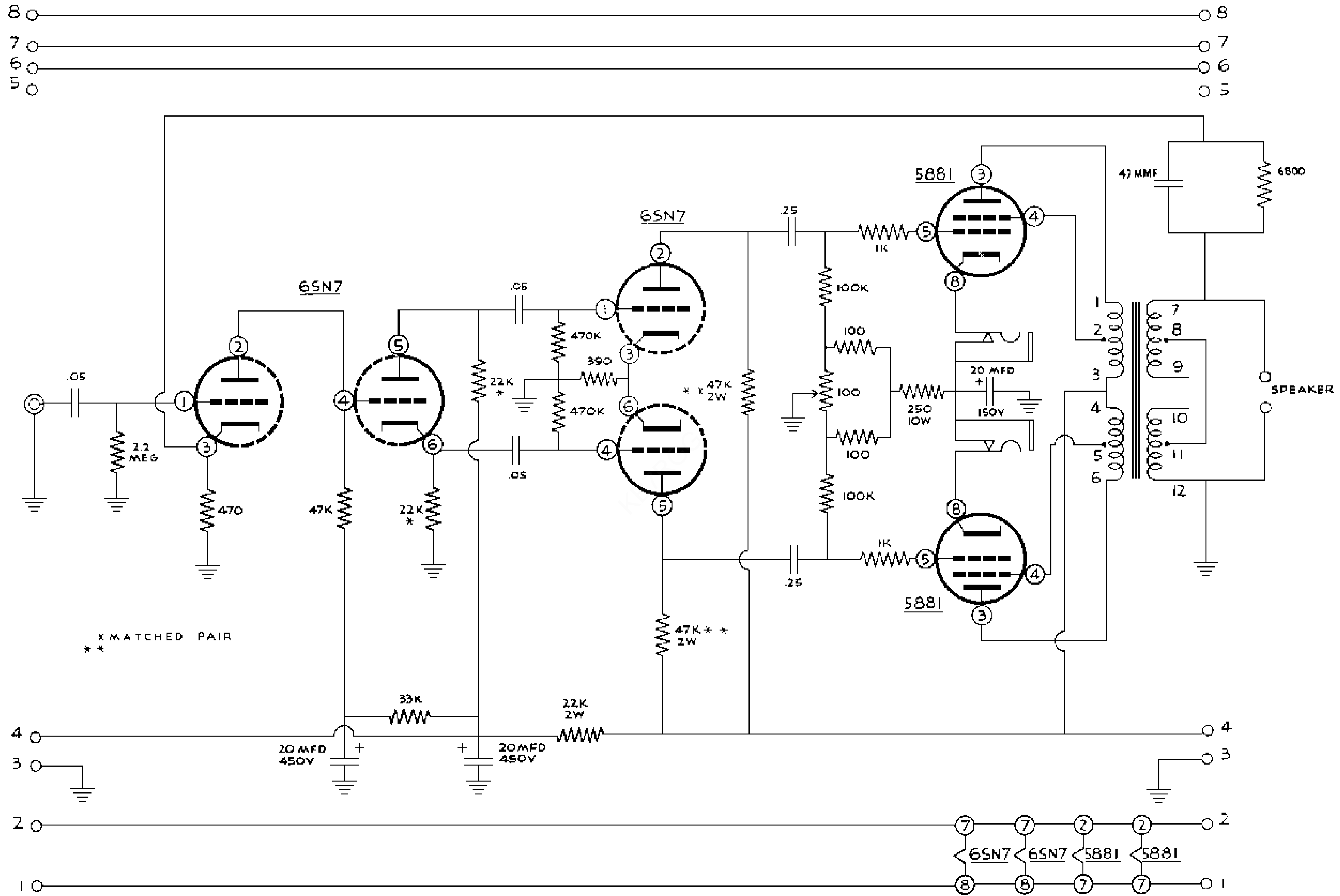
Heathkit MODEL W-2 AMPLIFIER CIRCUIT DIAGRAM
