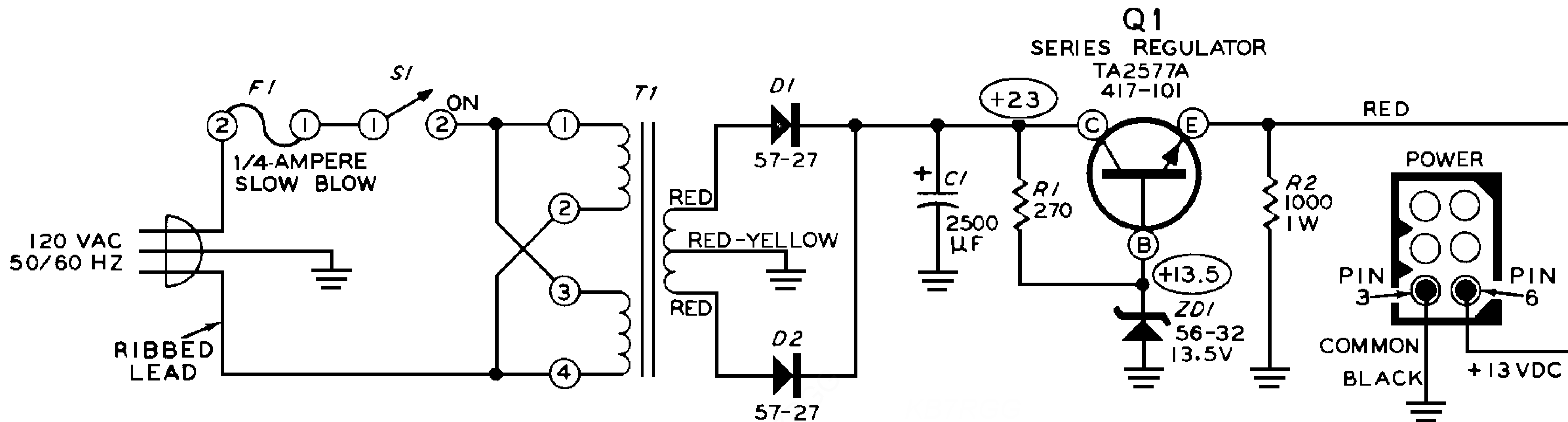
SCHEMATIC OF THE HEATHKIT® ACCESSORY POWER SUPPLY MODEL HWA-7-1
