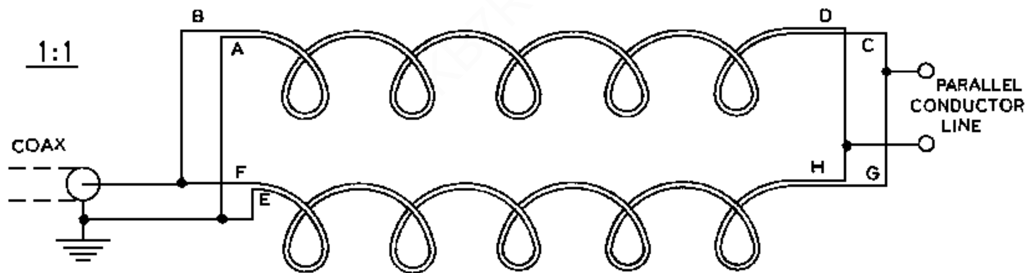
SCHMATIC HEATHKIT BALUN COIL MODEL B-1
